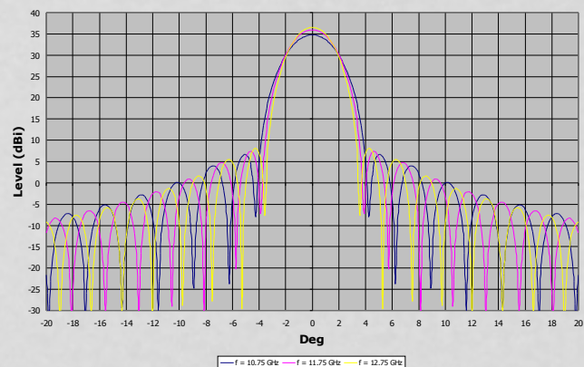
Radiation Patterns (Horizontal Plane)
